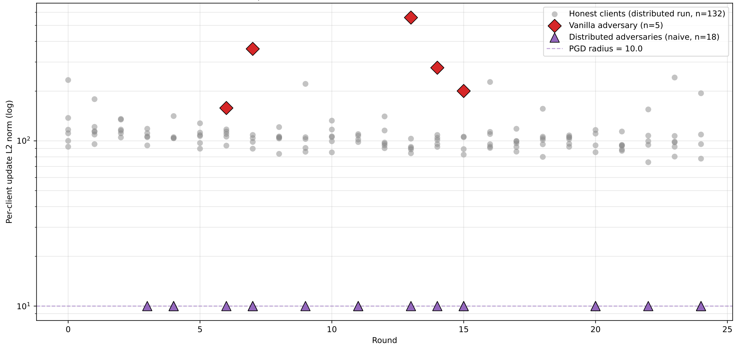
Per-client update norms: vanilla vs. distributed adversaries vs. honest band
