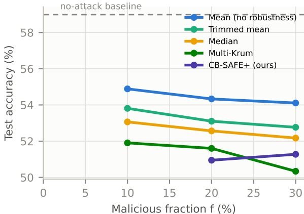
backdoor attack, robust rules across k=10 cluster sums (c=3)
