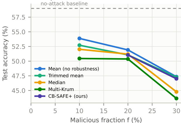
labelflip attack, robust rules across k=10 cluster sums (c=3)
