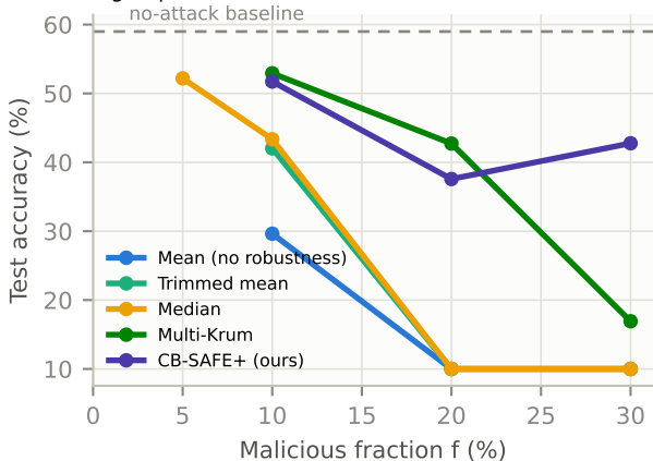
signflip attack, robust rules across k=10 cluster sums ( c=3 )
