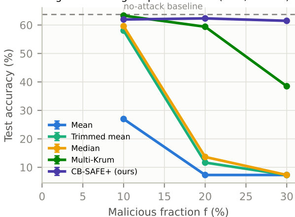
Edge-IIoTset: sign-flip robustness ( c=3 , 1 seed)
