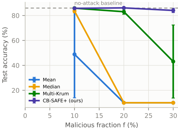
FashionMNIST: sign-flip robustness ( c=3 , 3 seeds)
