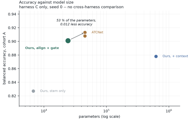
Figure 3: Balanced accuracy against parameter count on cohort A, harness C only. The proposed configuration sits 0.012 below ATCNet at 53% of its parameters. No point from the other harness appears here.
