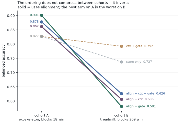
Figure 5: The same five arms on both cohorts. Solid lines use alignment, dashed lines do not. The ordering does not compress between cohorts — it inverts, and the three alignment arms cross below both alignment-free arms.
