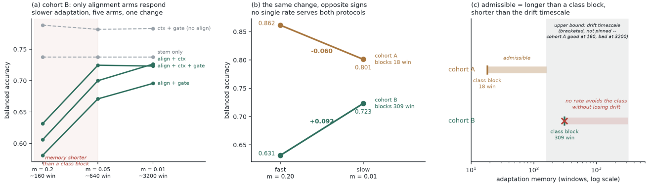
Figure 6: The adaptation rate condition. (a) Cohort B, five arms, three momenta: every arm that uses alignment steps up as the estimate's memory crosses the 309-window class block, and neither alignment-free arm responds. (b) The same change applied to both cohorts at matched estimator version produces opposite signs, so no single rate serves both protocols. (c) The admissible band of (2), bounded below by the class-block duration and above by the drift timescale: wide for cohort A, empty for cohort B.
