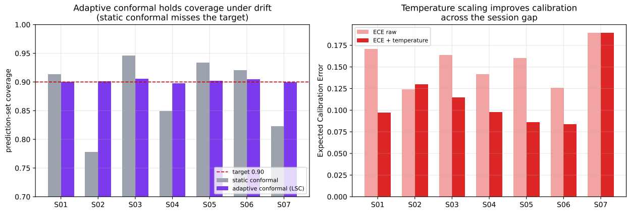
Fig. 3. Full CALM-Net across seven subjects. Left: adaptive conformal inference holds coverage at the 0.90 target under cross-session drift, where static conformal misses it. Right: temperature scaling lowers calibration error across the session gap.
