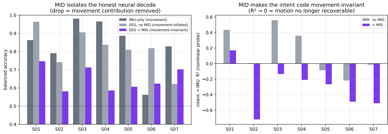
Fig. 2. Motion-invariant disentanglement across seven subjects. Left: balanced accuracy of the IMU-only baseline, the decoder without MID, and with MID. Right: recoverability of the IMU descriptor from the intent code, under the original cross-split probe; see Section VI for the corrected estimate.
