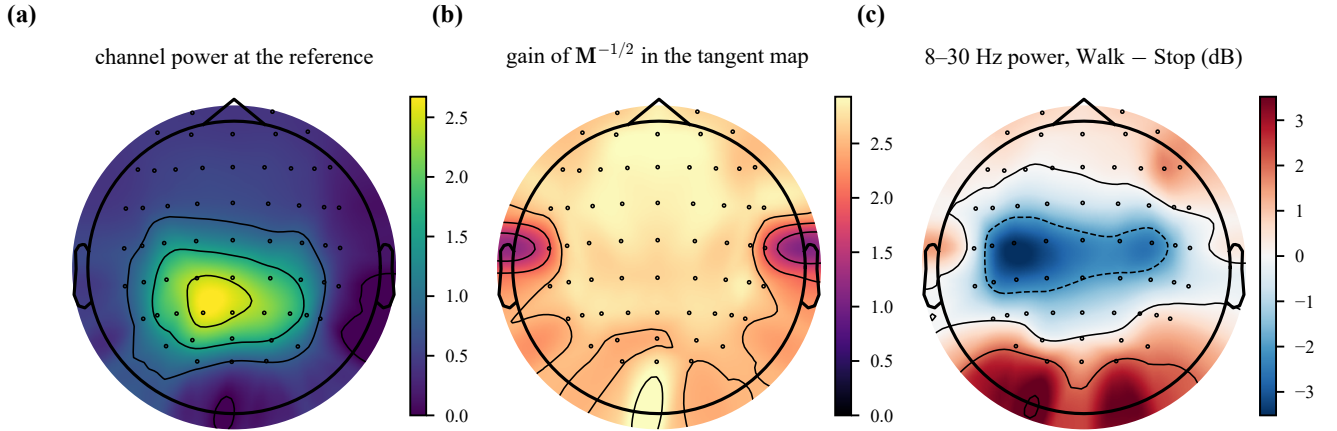
Figure 3: Where the branch's reference acts, and what the classes differ by. One cohort A participant, first three sessions, montage from the recorded channel names. The reference is built by the branch itself, with its own shrinkage and per-window trace normalisation, so these are the quantities the reported model holds at inference. (a) Channel power at the reference. (b) Per-channel gain of M^{-1/2} , which the tangent map applies: the frontocentral midline is amplified most (AFz, Fz, F2 at 2.9) and the temporal sites most exposed to jaw and neck muscle are amplified least (T7 and T8 at 1.9). (c) Absolute 8–30 Hz power, Walk minus Stop. The decrease is over left sensorimotor cortex (C3 -3.5 dB, C1 -3.0 , CP3 -2.8 ), the topography and sign expected of mu and beta desynchronisation, and the increase is occipital (O1 and O2 at +2.1 ), consistent with optic flow during walking. Gross movement artefact would raise power during walking rather than lower it over sensorimotor cortex, so the sign of this contrast argues against an artefact account without settling it. It is one participant, and a power contrast is not an artefact rejection (Section 8).
