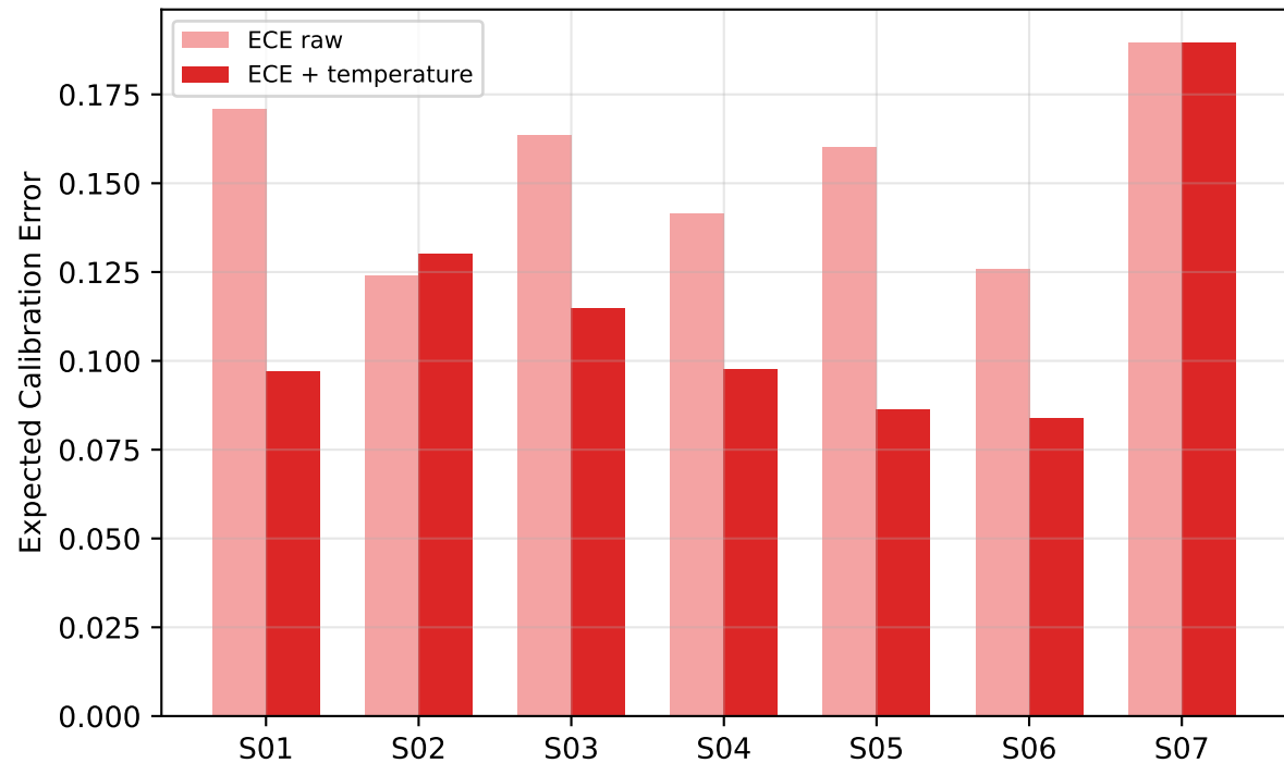
Temperature scaling improves calibration across the session gap
