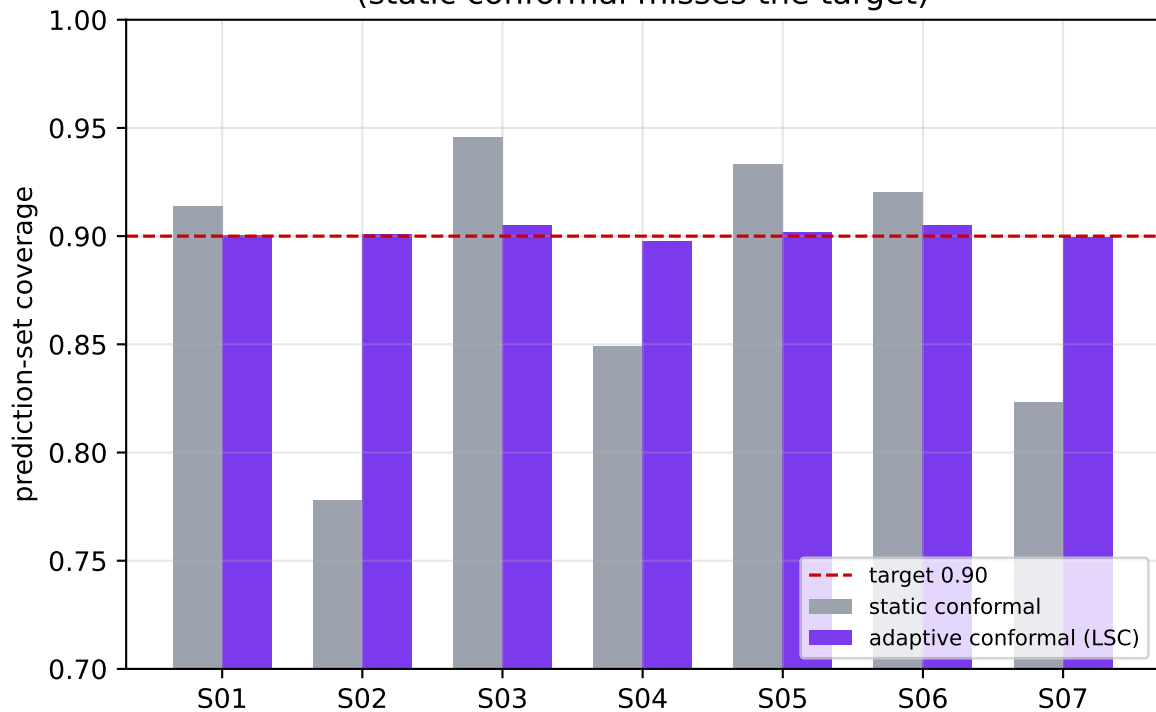
Adaptive conformal holds coverage under drift (static conformal misses the target)
