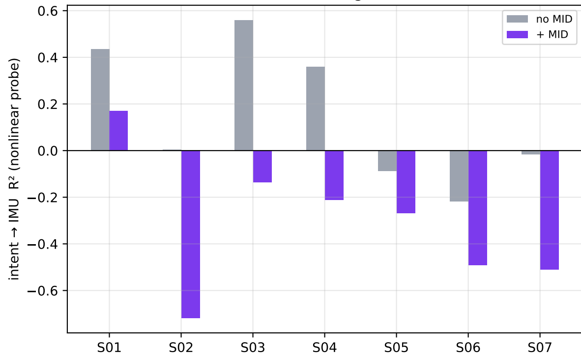
MID makes the intent code movement-invariant ( R^2 \rightarrow 0 = motion no longer recoverable)
