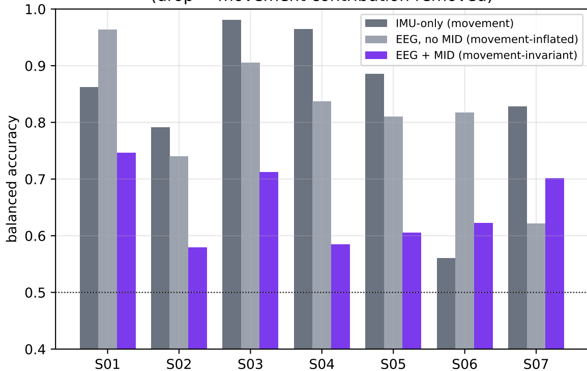
MID isolates the honest neural decode (drop = movement contribution removed)
