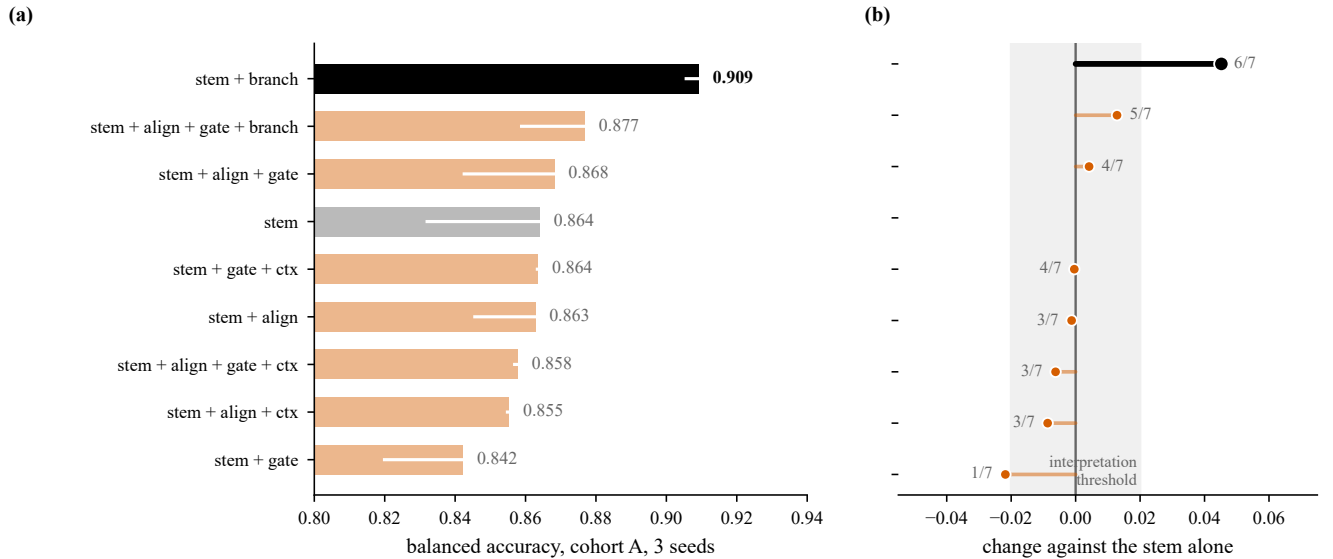
Figure 3: Ablation of the reported model on cohort A, three data-split seeds. (a) Balanced accuracy by configuration; the reported model is solid, the stem it is built on is grey, and every configuration containing a component that was tested and not retained is faded. White bars are one standard deviation across seeds. (b) The same arms as a change against the stem alone, paired across participants with seeds averaged within participant; the annotation gives how many participants improved and the shaded band is the 0.02 interpretation threshold. The branch is the only component that raises accuracy. Nothing built from the alignment layer, the gate or the cross-epoch transformer improves on the stem by more than 0.005, and the gate alone is 0.022 below it.
