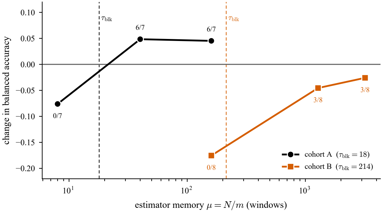
Figure 7: The rate condition, measured by manipulation rather than by comparing cohorts. Each point moves only the estimator memory \mu = N/m , with the architecture, the data and every other setting fixed; dashed verticals mark each cohort's class-block length and annotations give how many participants improved. On cohort A the branch gains +0.045 and +0.048 at memories of 160 and 40 windows, both above its 18-window block, and reverses to -0.076 in every participant at a memory of 8, below it. On cohort B, whose blocks are 214 windows, the effect recovers monotonically as the memory is raised past them but does not become positive. The effect therefore appears and disappears as \mu crosses \tau_{\text{blk}} , which is the causal form of the comparison Fig. 8 makes across cohorts.
