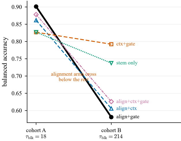
Figure 5: The same five arms on both cohorts, single seed. None of these arms is the reported model; they are the components of Section 4.3. Solid heavy black is the best of them on cohort A; the other alignment-using arms are dashed in colour, and the two alignment-free arms are dashed and dotted. The three alignment arms cross below both alignment-free arms, so the ordering inverts instead of compressing.
