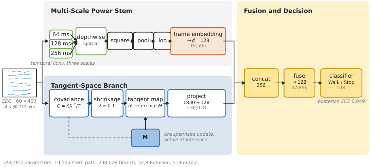
Figure 1: The reported decoder. A window enters both paths. The stem applies three temporal resolutions with depthwise spatial filters, squares, pools and takes the logarithm, giving log band power per channel. The branch forms the window's covariance, shrinks it, maps it to the tangent space at a running reference and projects the result. The reference update (dashed) uses no labels and stays active at inference, which is what lets the representation follow a changing session and also what makes it fail where a class block outlasts one update (Section 6.3). Parameter counts are exact and sum to the total.
