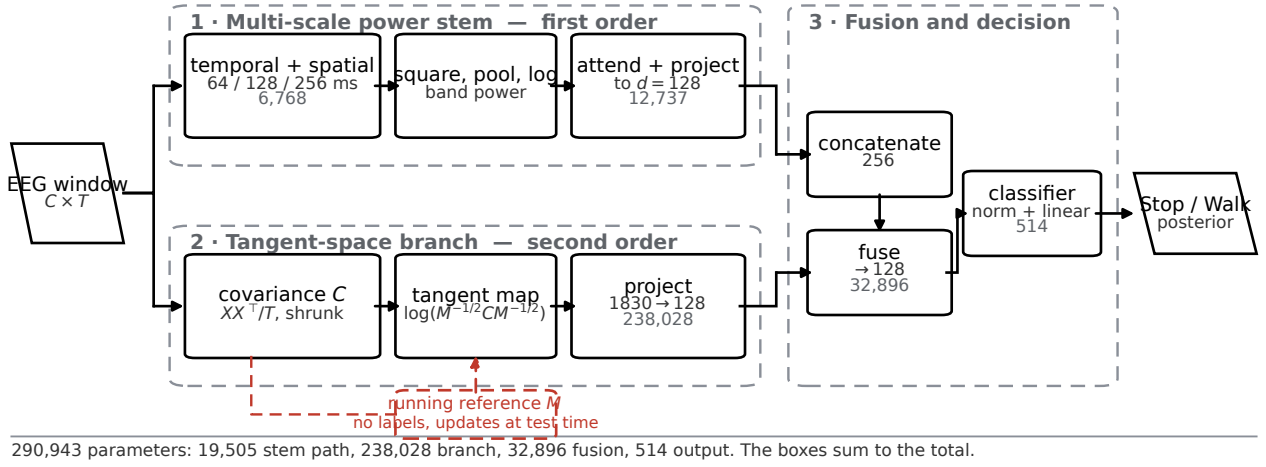
Figure 1: The reported decoder. A window enters both paths. The stem applies three temporal resolutions with depthwise spatial filters, squares, pools and takes the logarithm, giving log band power per channel. The branch forms the window’s covariance, shrinks it, maps it to the tangent space at a running reference and projects the result. The reference update (dashed) uses no labels and stays active at inference, which is what lets the representation follow a changing session and also what makes it fail where a class block outlasts one update (Section 6.3). Parameter counts are exact and sum to the total.
