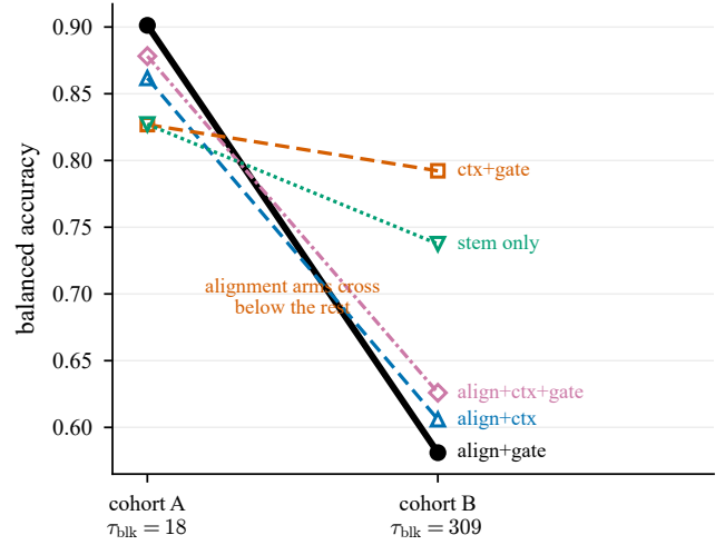
Figure 4: The same five arms on both cohorts, single seed. Solid heavy black is the proposed configuration; the other alignment-using arms are dashed in colour, and the two alignment-free arms are dashed and dotted. The three alignment arms cross below both alignment-free arms, so the ordering inverts instead of compressing.
