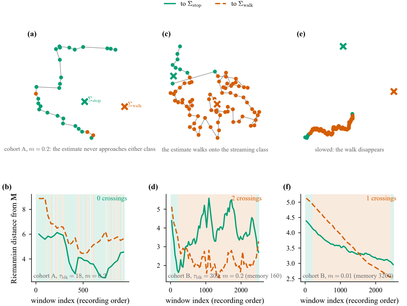
Figure 5: The running covariance estimate and the streaming class, one participant per cohort (cohort A sub-01, cohort B SL01). Top row: class covariances (crosses) and the estimate's path in recording order, projected to two dimensions by multidimensional scaling on the affine-invariant Riemannian distance and coloured by the streaming class. Bottom row: distance from the estimate to each class covariance against window index, with the background shaded by the streaming class. (a,b) Cohort A, \tau_{\text{blk}} = 18 , m = 0.2 : the estimate stays closer to the stop covariance throughout and approaches neither class. (c,d) Cohort B, \tau_{\text{blk}} = 309 , m = 0.2 : the estimate starts near the stop covariance, moves to the walk covariance when the walk block begins, and the two distances swap back when stop returns. (e,f) Cohort B at m = 0.01 : the estimate moves toward the walk covariance more slowly and crosses over once, late in the recording. [In-panel labels to be regenerated: text overlaps the curves in (b), (d) and (f).]
