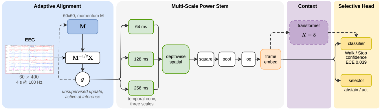
Figure 1: The decoder. The adaptive alignment layer maintains a running spatial covariance and whitenes by it; its update path (dashed, left) uses no labels and remains active at inference, which is what separates it from a normalisation layer. The cross-epoch context pathway is optional and accounts for 594,816 of the 618,997 parameters of the full configuration, so the default configuration omits it and uses 24,181. Parameter counts are exact and sum to the total.
