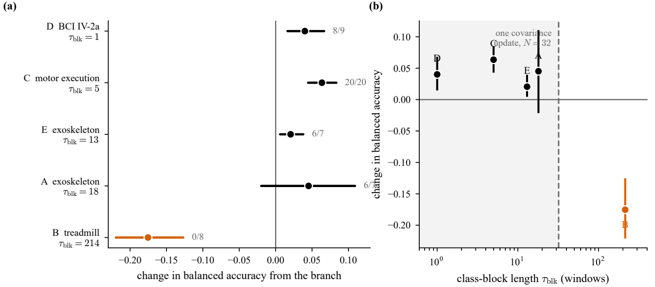
Figure 8: The branch on every cohort. (a) Change in balanced accuracy against the stem alone, paired across participants with seeds averaged within participant; bars are 95 % intervals from a paired bootstrap over participants, and the annotation gives how many participants improved. Cohorts are ordered by the class-block length of their protocol. (b) The same five effects against that block length, with the number of windows averaged into one covariance update drawn as a dashed line. The branch helps on every cohort whose blocks are shorter than one update and fails on the only one whose blocks are longer. Both axes of (b) are fixed before training: the block length is read from the labels and the update size is the batch size, so the separation uses no accuracy.
