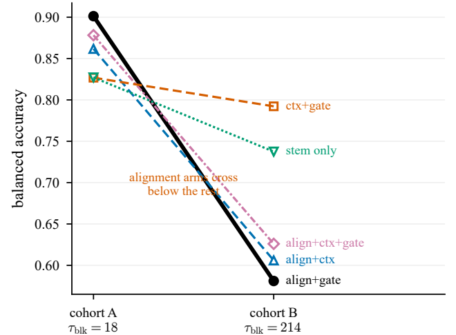
Figure 5: The same five arms on both cohorts, single seed. None of these arms is the reported model; they are the components of Section 4.3. Solid heavy black is the best of them on cohort A; the other alignment-using arms are dashed in colour, and the two alignment-free arms are dashed and dotted. The three alignment arms cross below both alignment-free arms, so the ordering inverts instead of compressing.
