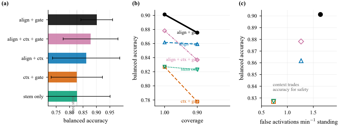
Figure 3: Component ablation on cohort A, seed 0, over the components of Section 4.3 that were tested and are not in the reported model. It is retained because the ablation is reported against these arms; the reported model appears in Table 12 and Fig. 8. (a) Balanced accuracy by arm; error bars are \pm 1 SD across the 7 participants; seed variation is reported separately in Table 10. (b) Balanced accuracy at 90% coverage, obtained by declining the least-confident 10% of windows. It sits below full-coverage accuracy for every arm with a trained gate. (c) Balanced accuracy against spurious activations per minute of standing, showing the cross-epoch context as a selectable operating point. Three-seed values under the current estimator are in Table 4.
