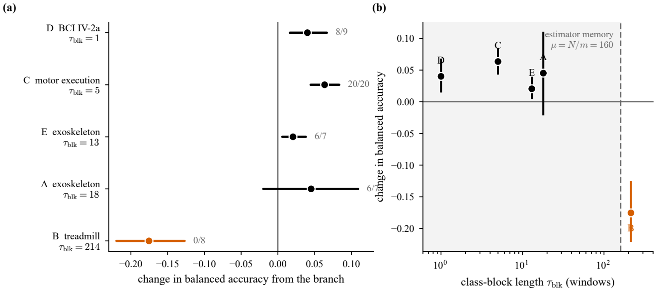
Figure 5: The branch on every cohort. (a) Change in balanced accuracy against the stem alone, paired across participants with seeds averaged within participant; bars are 95 % intervals from a paired bootstrap over participants, and the annotation gives how many participants improved. Cohorts are ordered by the class-block length of their protocol. (b) The same five effects against that block length, with the estimator memory drawn as a dashed line. The branch helps on every cohort whose blocks are shorter than one update and fails on the only one whose blocks are longer. Both axes of (b) are fixed before training: the block length is read from the labels and the memory is fixed by the optimiser settings, so the separation uses no accuracy. Table 13 moves the memory directly and crosses this boundary in both directions on one cohort.
