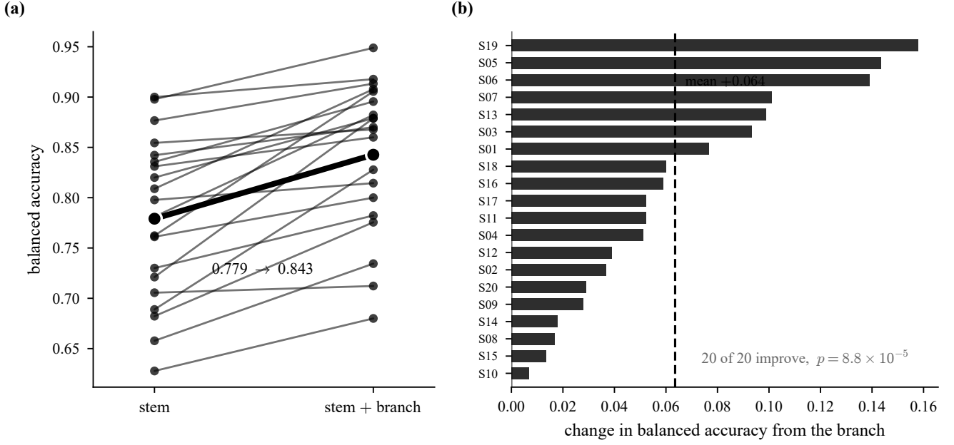
Figure 4: The branch on cohort C, which was held out from every design decision, three seeds averaged within participant. (a) Each line is one of the twenty participants, stem on the left and stem plus branch on the right; the heavy line is the mean. (b) The same differences sorted, with the mean dashed. Every participant improves, by +0.007 to +0.158, p = 8.8 \times 10^{-5} . This is the cohort that carries the accuracy claim: cohorts A and E are smaller and their intervals are correspondingly wider.
