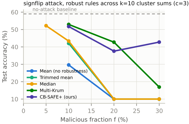
Fig. 6. Sign-flip attack ( \gamma=5 ): accuracy vs. malicious fraction across aggregation rules over k=10 cluster sums ( c=3 ). Coordinate-wise rules collapse at the contamination boundary the (1-f)^c law predicts; vector selection degrades gracefully; CB-SAFE+ identifies and excludes the attackers.
