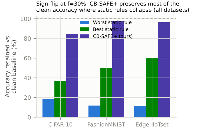
Fig. 8. Sign-flip at f=30\% : fraction of clean-baseline accuracy retained by the worst static rule, the best static rule, and CB-SAFE+, on every dataset. CB-SAFE+ preserves 84–97% where static rules keep 12–60%.
