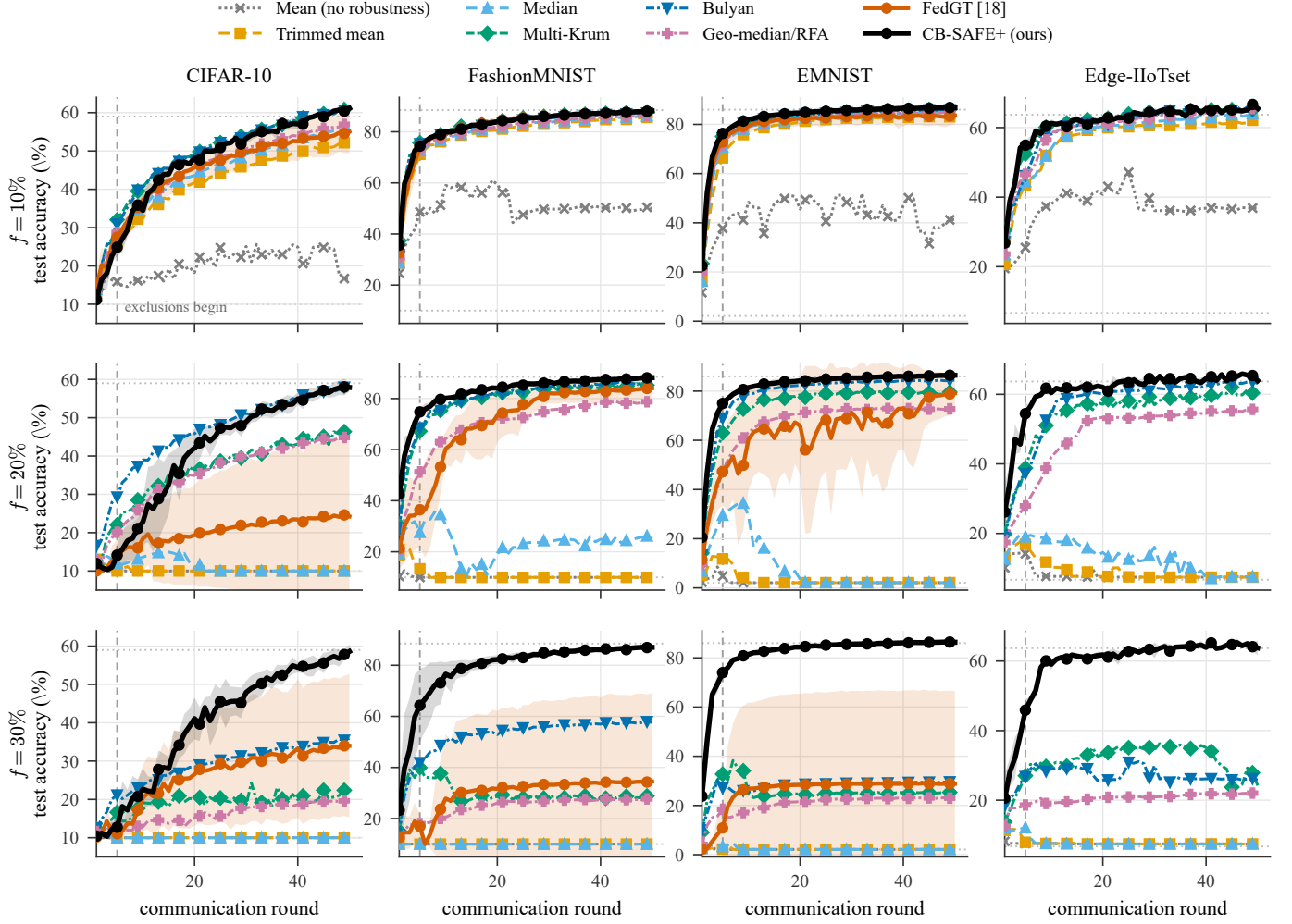
Fig. 6. Training dynamics under sign-flip: test accuracy vs round, eight rules across four datasets (columns) \times malicious fraction f (rows). Mean over 3 seeds; \pm 1 SD bands for CB-SAFE+ and FedGT (real BCJR [18]). Dashed line: warmup W=5 .
