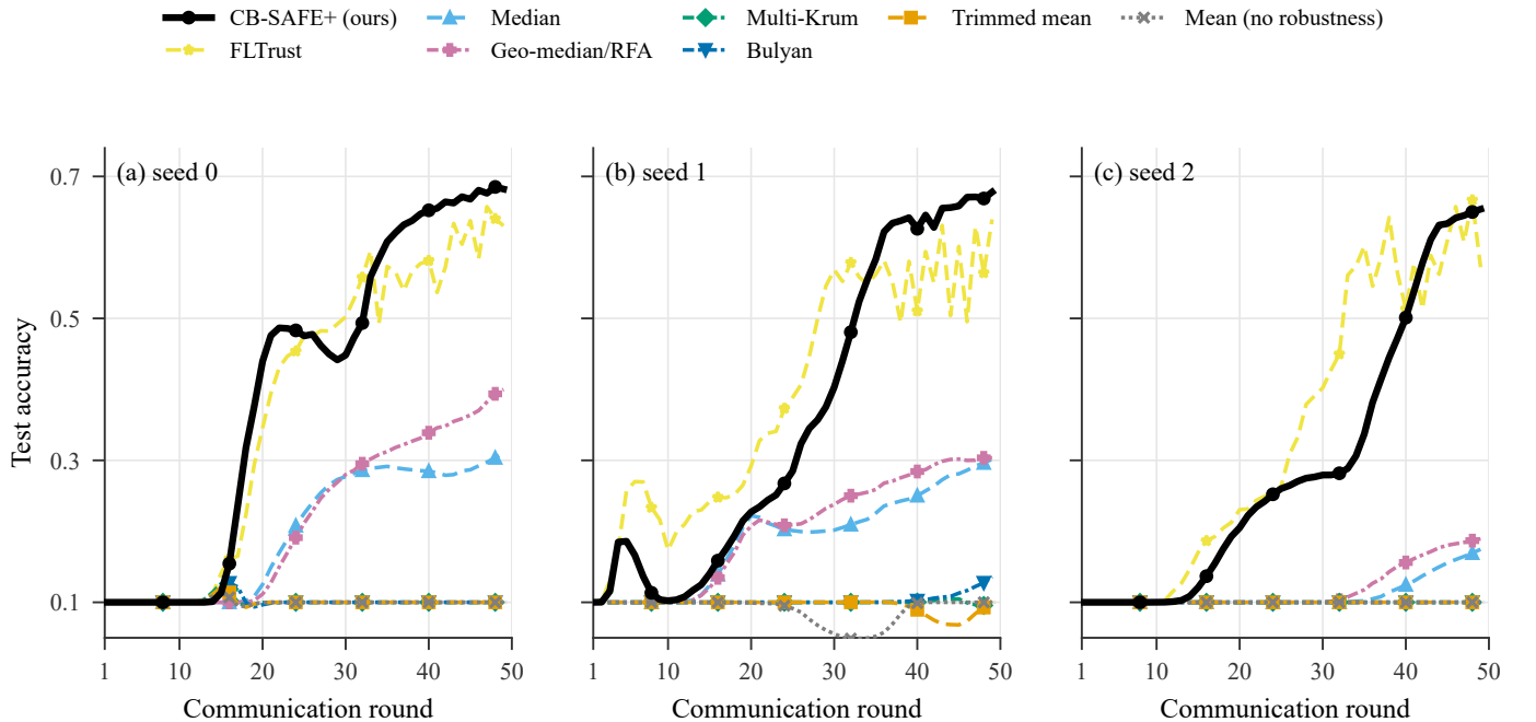
Fig. 3. Test accuracy versus communication round at N=500 (FashionMNIST, sign-flip f=0.2 , 50 rounds), one panel per seed (three seeds), all eight aggregation rules that admit a configuration at this scale (FedGT excluded; see text). CB-SAFE+ (heavy black) recovers to \sim 66\% ; the coordinate-wise rules stay laundered near chance (10%); FLTrust leads early but plateaus lower. Recovery begins only after attacker exclusion ( \sim round 15–20), so a 30-round budget would truncate every curve mid-climb.
