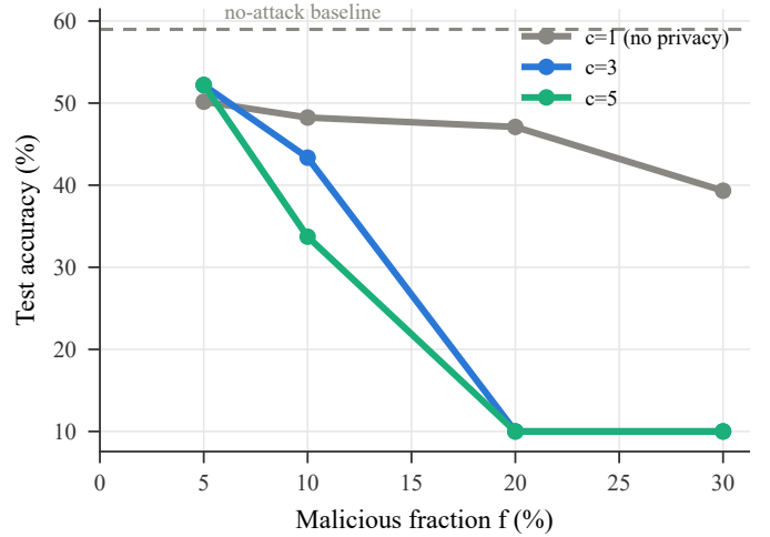
Fig. 7. The privacy-robustness dial, measured: median-rule accuracy under sign-flip for c \in \{1, 3, 5\} . Larger anonymity sets shift the breakdown frontier left, as (1-f)^c predicts; at f=5\% privacy costs nothing.
