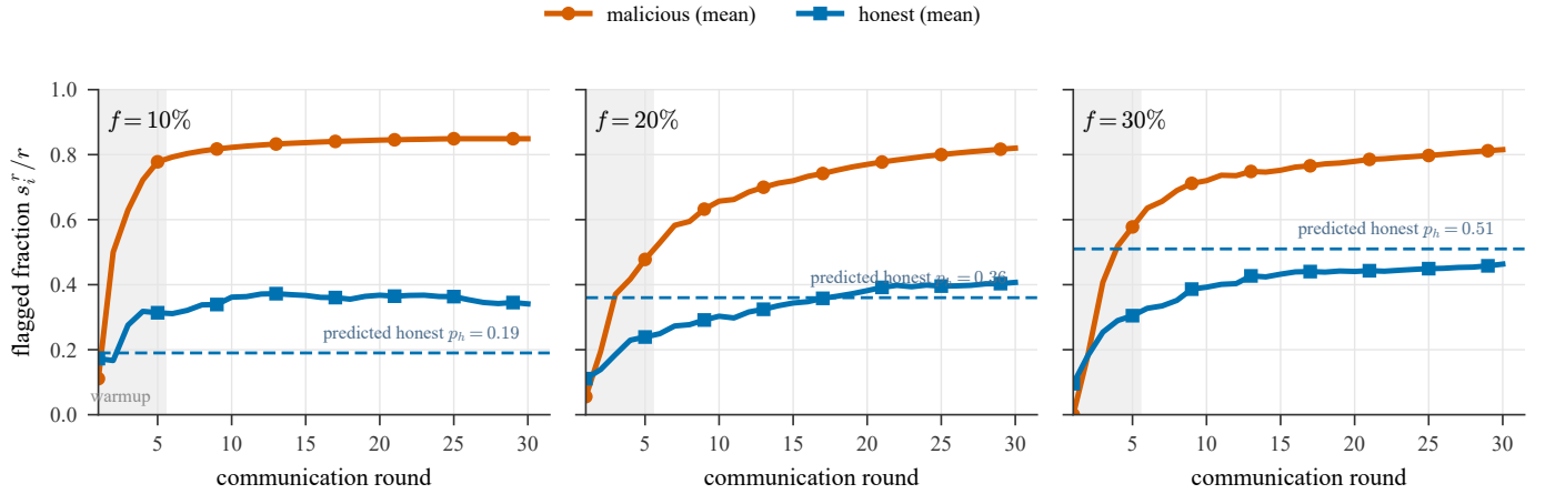
Fig. 6. Temporal suspicion separation (CB-SAFE+ on CIFAR-10): population-mean flagged fraction s_i^r / r of malicious versus honest clients over rounds, for each malicious fraction f (mean over 3 seeds). The two populations separate within a few rounds, so attackers are identified from group-level observations alone (Eqs. (4)–(6)). The dashed line is the predicted honest co-clustering rate p_h = 1 - (1 - f)^{c-1} (Eq. (5)); the loss probe adds a few honest flags at low f . Exclusion uses an adaptive gap between the two populations rather than a fixed threshold; the warmup window is shaded.
