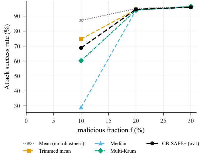
Fig. 4. Backdoor attack success rate vs. malicious fraction. No sum-level rule suppresses the trigger (median at f=0.1 partially excepted); backdoored sums help the main task and evade loss/direction probes, the honest scope limit of robustness under secure aggregation.
