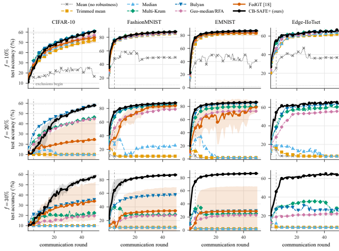
Fig. 5. Training dynamics under sign-flip: test accuracy vs round, eight rules across four datasets (columns) \times malicious fraction f (rows). Mean over 3 seeds; \pm 1 SD bands for CB-SAFE+ and FedGT (real BCJR [18]). Dashed line: warmup W=5 .
