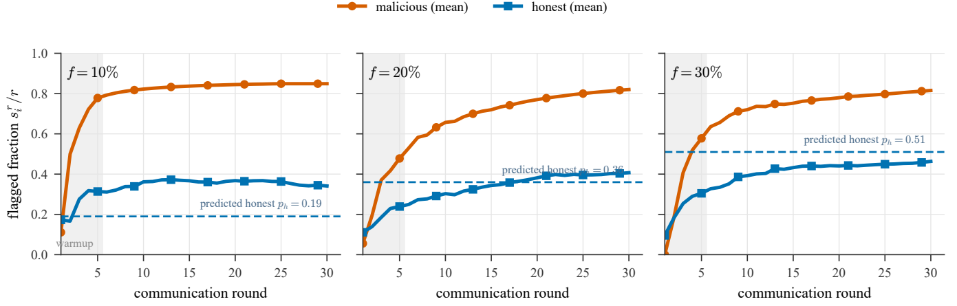
Fig. 7. Temporal suspicion (CB-SAFE+, CIFAR-10): mean flagged fraction s_i^T/r for malicious vs honest clients, per fraction f (3 seeds). Dashed: predicted honest rate p_h = 1 - (1 - f)^{c-1} ; warmup shaded.
