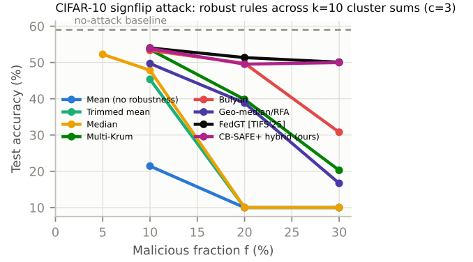
Fig. 6. Sign-flip attack ( \gamma=5 ) on CIFAR-10: test accuracy vs. malicious fraction across eight aggregation rules over k=10 cluster sums ( c=3 , mean of three seeds). Coordinate-wise rules (mean, trimmed mean, median) and the geometric median (RFA) collapse to chance at the (1-f)^c contamination boundary; vector selection (Multi-Krum, Bulyan) degrades gracefully then falls; and only the two group-testing methods, CB-SAFE+ hybrid and FedGT, hold near the clean baseline across all f . (FLTrust omitted: its f=0.1 point is still computing.)
