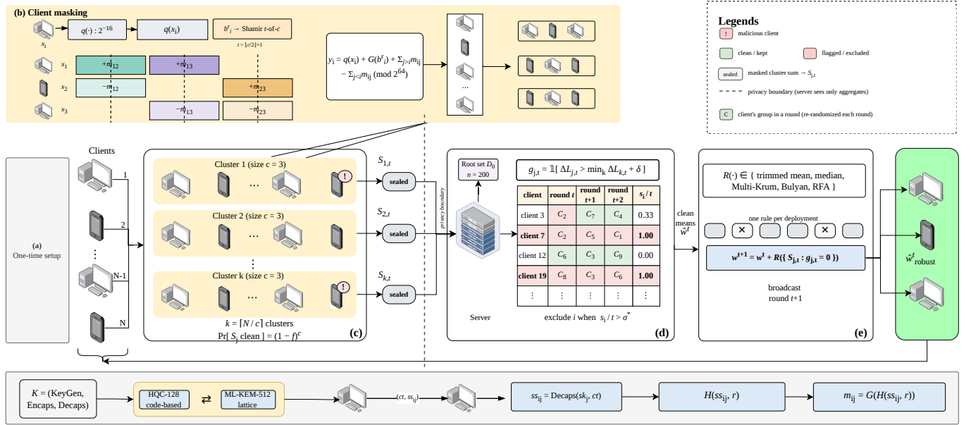
Fig. 1. CB-SAFE, one training round end to end: one-time HQC key setup, within-cluster masked aggregation (the server sees only the k cluster sums), and the CB-SAFE+ flag/exclude stage.
