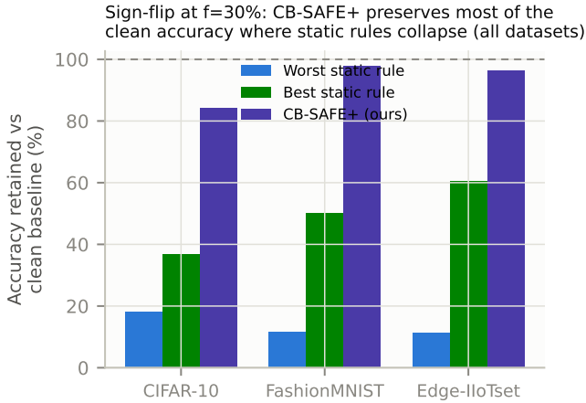
Fig. 8. Sign-flip at f=30\% : fraction of clean-baseline accuracy retained by the worst static rule, the best static rule, and CB-SAFE+, on every dataset. CB-SAFE+ preserves 84–97% where static rules keep 12–60%.
