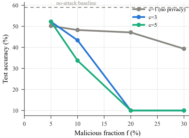
Fig. 11. The privacy-robustness dial, measured: median-rule accuracy under sign-flip for c \in \{1, 3, 5\} . Larger anonymity sets shift the breakdown frontier left, as (1 - f)^c predicts; at f=5\% privacy costs nothing.
