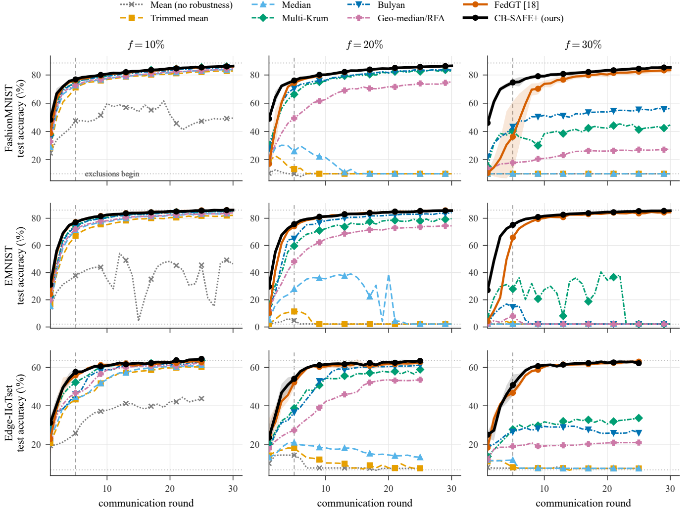
Fig. 9. Training dynamics under the sign-flip attack: test accuracy versus communication round for eight aggregation rules, across three datasets (rows) and malicious fractions f (columns). Curves are the mean over 3 seeds (single seed for EMNIST); shaded bands are \pm 1 SD for CB-SAFE+ and FedGT. The dashed vertical marks the warmup W=5 after which exclusions begin; dotted lines mark chance and the no-attack baseline. Coordinate-wise rules and the geometric median decay progressively to chance at f \geq 0.2 , whereas CB-SAFE+ dips during warmup and then recovers as attackers are excluded, tracking or exceeding FedGT. CIFAR-10 (a statistical tie with FedGT) is reported in Table V.
