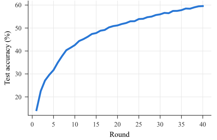
Fig. 5. Test accuracy of FedAvg on non-IID CIFAR-10; CB-SAFE's secure aggregates (HQC and ML-KEM) are numerically equivalent to plain aggregation, so the accuracy curve is shared by all three configurations.
