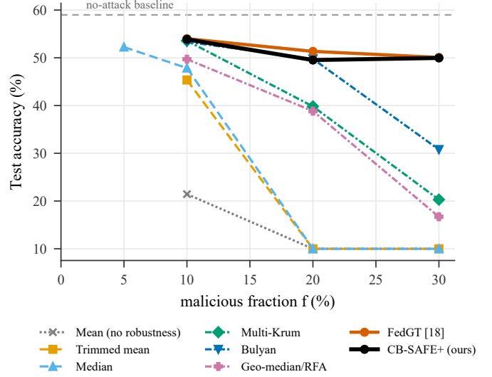
Fig. 6. Sign-flip attack ( \gamma=5 ) on CIFAR-10: test accuracy vs. malicious fraction across eight aggregation rules over k=10 cluster sums ( c=3 , mean of three seeds). Coordinate-wise rules (mean, trimmed mean, median) and the geometric median (RFA) collapse to chance at the (1-f)^c contamination boundary; vector selection (Multi-Krum, Bulyan) degrades gracefully then falls; and only the two group-testing methods, CB-SAFE+ hybrid and FedGT, hold near the clean baseline across all f . (FLTrust omitted: its f=0.1 point is still computing.)
