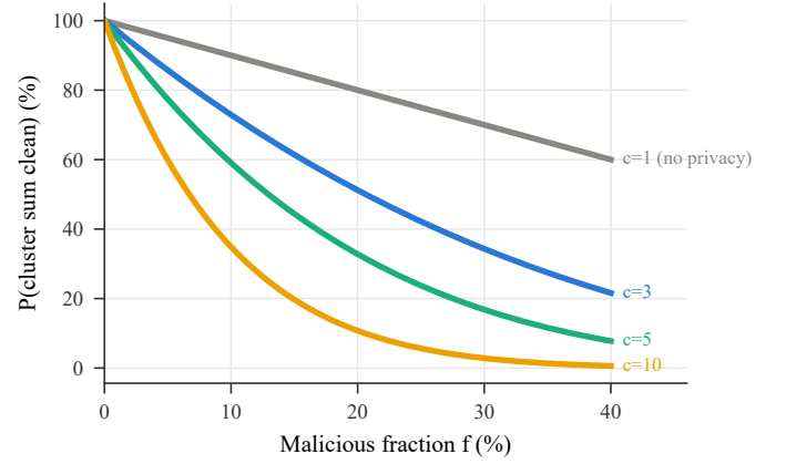
Fig. 12. The privacy-robustness dial, analytically: the anonymity set grows with cluster size c , while the probability that a cluster sum is uncontaminated decays as (1 - f)^c .
