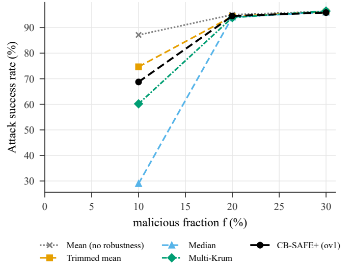
Fig. 6. Backdoor attack success rate vs. malicious fraction. No sum-level rule suppresses the trigger (median at f=0.1 partially excepted): backdoored sums help the main task and evade loss/direction probes, the honest scope limit of robustness under secure aggregation.
