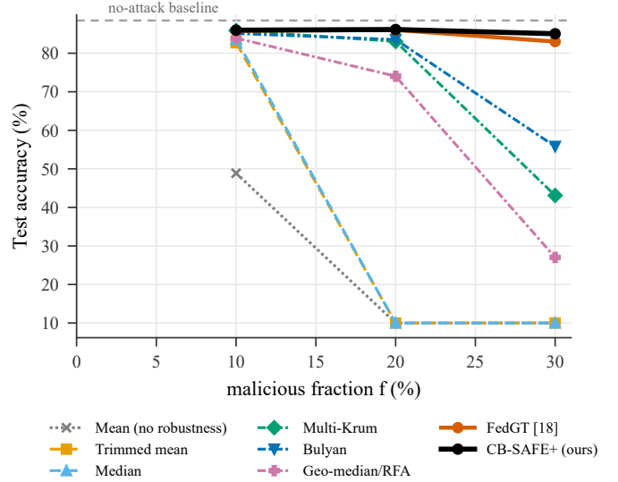
Fig. 5. Sign-flip attack ( \gamma=5 ) on FashionMNIST: test accuracy vs. malicious fraction across eight aggregation rules over k=10 cluster sums ( c=3 , mean of three seeds). Coordinate-wise rules (mean, trimmed mean, median) and the geometric median (RFA) collapse toward chance at the (1-f)^c contamination boundary; vector selection (Multi-Krum, Bulyan) degrades then falls; only CB-SAFE+ and FedGT hold near the clean baseline across all f , with CB-SAFE+ highest at f=0.3 . CIFAR-10 (a statistical tie with FedGT) and the other datasets are reported in Table V.
