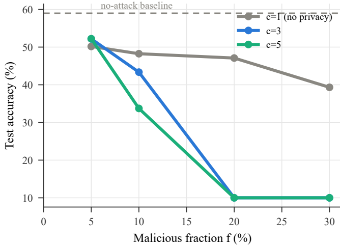
Fig. 9. The privacy-robustness dial, measured: median-rule accuracy under sign-flip for c \in \{1, 3, 5\} . Larger anonymity sets shift the breakdown frontier left, as (1 - f)^c predicts; at f=5\% privacy costs nothing.
