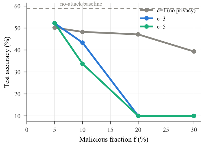
Fig. 8. Privacy-robustness dial: median-rule accuracy under sign-flip for c \in \{1, 3, 5\} (CIFAR-10).
