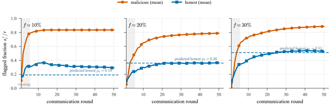
Fig. 8. Temporal suspicion (CB-SAFE+, CIFAR-10): mean flagged fraction s_i^T/r for malicious vs honest clients, per fraction f (3 seeds). Dashed: predicted honest rate p_h = 1 - (1 - f)^{c-1} ; warmup shaded.
