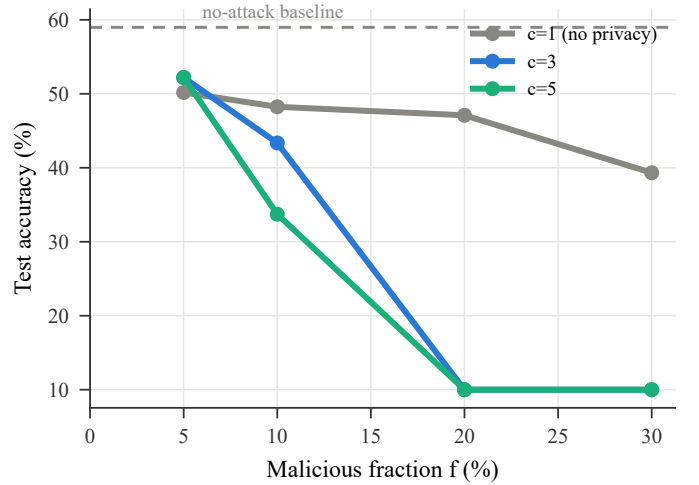
Fig. 10. The privacy-robustness dial, measured: median-rule accuracy under sign-flip for c \in \{1, 3, 5\} . Larger anonymity sets shift the breakdown frontier left, as (1 - f)^c predicts; at f=5\% privacy costs nothing.
