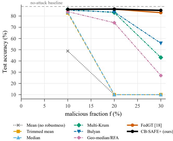
Fig. 6. Sign-flip attack ( \gamma=5 ) on FashionMNIST: test accuracy vs. malicious fraction across eight aggregation rules over k=10 cluster sums ( c=3 , mean of three seeds). Coordinate-wise rules (mean, trimmed mean, median) and the geometric median (RFA) collapse toward chance at the (1-f)^c contamination boundary; vector selection (Multi-Krum, Bulyan) degrades then falls; only CB-SAFE+ and FedGT hold near the clean baseline across all f , with CB-SAFE+ highest at f=0.3 . CIFAR-10 (a statistical tie with FedGT) and the other datasets are reported in Table V.
