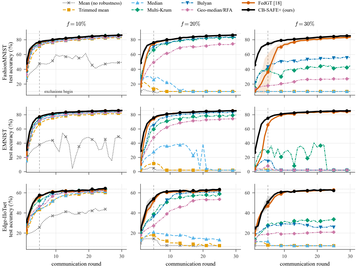
Fig. 8. Training dynamics under the sign-flip attack: test accuracy versus communication round for eight aggregation rules, across three datasets (rows) and malicious fractions f (columns). Curves are the mean over 3 seeds (single seed for EMNIST); shaded bands are \pm 1 SD for CB-SAFE+ and FedGT. The dashed vertical marks the warmup W=5 after which exclusions begin; dotted lines mark chance and the no-attack baseline. Coordinate-wise rules and the geometric median decay progressively to chance at f \geq 0.2 , whereas CB-SAFE+ dips during warmup and then recovers as attackers are excluded, tracking or exceeding FedGT. CIFAR-10 (a statistical tie with FedGT) is reported in Table V.
