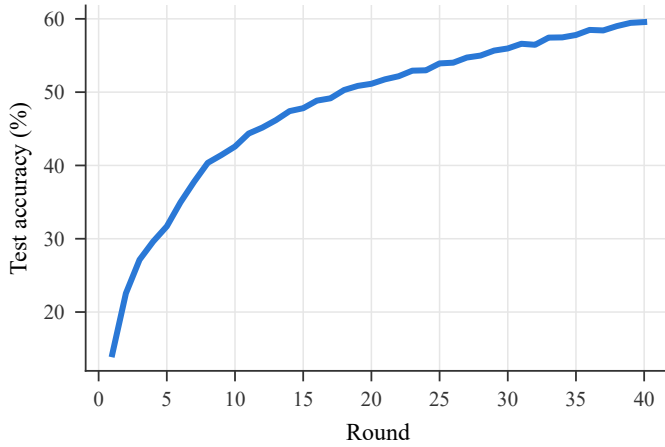
Fig. 5. Test accuracy of FedAvg on non-IID CIFAR-10; CB-SAFE's secure aggregates (HQC and ML-KEM) are numerically equivalent to plain aggregation, so the accuracy curve is shared by all three configurations.
