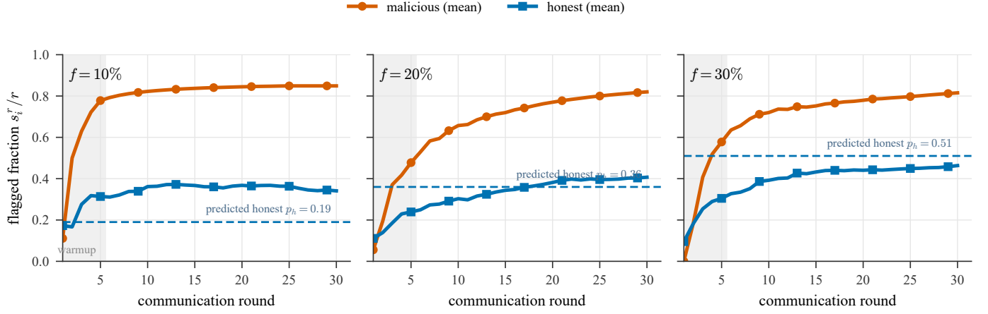
Fig. 9. Temporal suspicion separation (CB-SAFE+ on CIFAR-10): population-mean flagged fraction s_i^r/r of malicious versus honest clients over rounds, for each malicious fraction f (mean over 3 seeds). The two populations separate within a few rounds, so attackers are identified from group-level observations alone (Eqs. (4)–(6)). The dashed line is the predicted honest co-clustering rate p_h = 1 - (1 - f)^{c-1} (Eq. (5)); the loss probe adds a few honest flags at low f . Exclusion uses an adaptive gap between the two populations rather than a fixed threshold; the warmup window is shaded.
