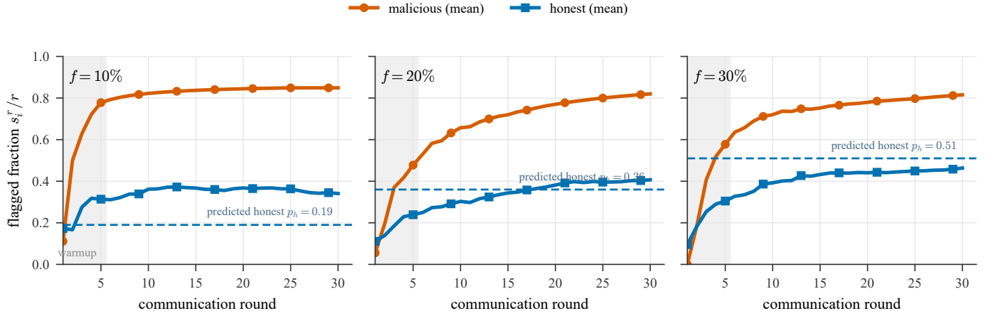
Fig. 8. Temporal suspicion separation (CB-SAFE+ on CIFAR-10): population-mean flagged fraction s_i^r / r of malicious versus honest clients over rounds, for each malicious fraction f (mean over 3 seeds). The two populations separate within a few rounds, so attackers are identified from group-level observations alone (Eqs. (4)–(6)). The dashed line is the predicted honest co-clustering rate p_h = 1 - (1 - f)^{c-1} (Eq. (5)); the loss probe adds a few honest flags at low f . Exclusion uses an adaptive gap between the two populations rather than a fixed threshold; the warmup window is shaded.
