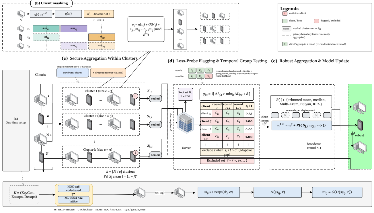
Fig. 1. CB-SAFE end-to-end pipeline: one-time code-based (HQC) key setup, per-round masked cluster aggregation, robust aggregation across cluster sums, and CB-SAFE+ temporal group-testing exclusion.
