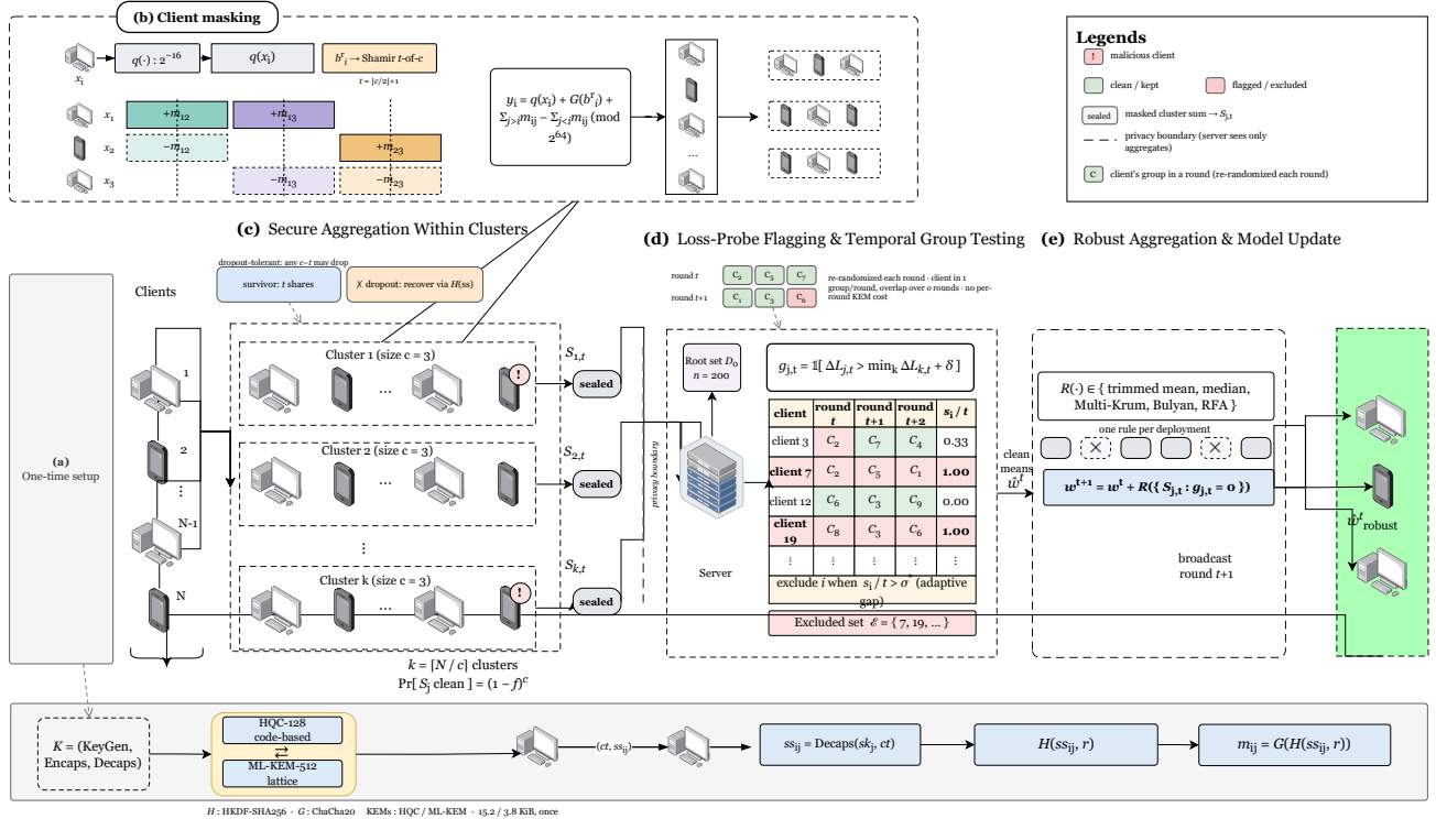
Fig. 1. CB-SAFE, one training round end to end: one-time HQC key setup, within-cluster masked aggregation (the server sees only the k cluster sums), and the CB-SAFE+ flag/exclude stage.
