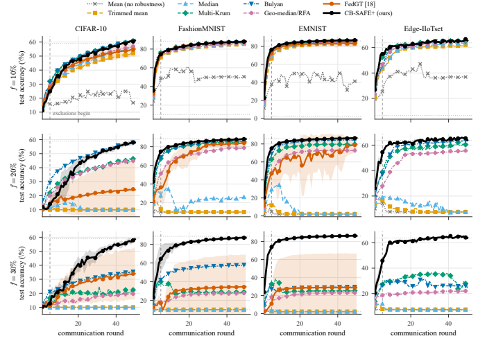
Fig. 6. Training dynamics under sign-flip: test accuracy vs. round, eight rules across four datasets (columns) \times malicious fraction f (rows). Mean over 3 seeds; \pm 1 SD bands for CB-SAFE+ and FedGT (real BCJR [18]). Dashed line: warmup W=5 .
