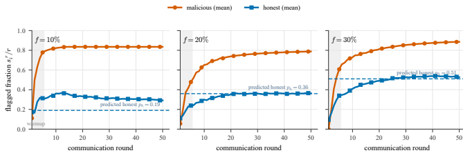
Fig. 8. Temporal suspicion (CB-SAFE+, CIFAR-10): mean flagged fraction s_i^r/r for malicious vs honest clients, per fraction f (3 seeds). Dashed: predicted honest rate p_h = 1 - (1 - f)^{c-1} ; warmup shaded.
