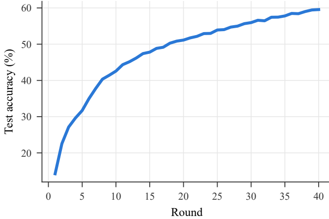
Fig. 6. Test accuracy of FedAvg on non-IID CIFAR-10; CB-SAFE’s secure aggregates (HQC and ML-KEM) are numerically equivalent to plain aggregation, so the accuracy curve is shared by all three configurations.
