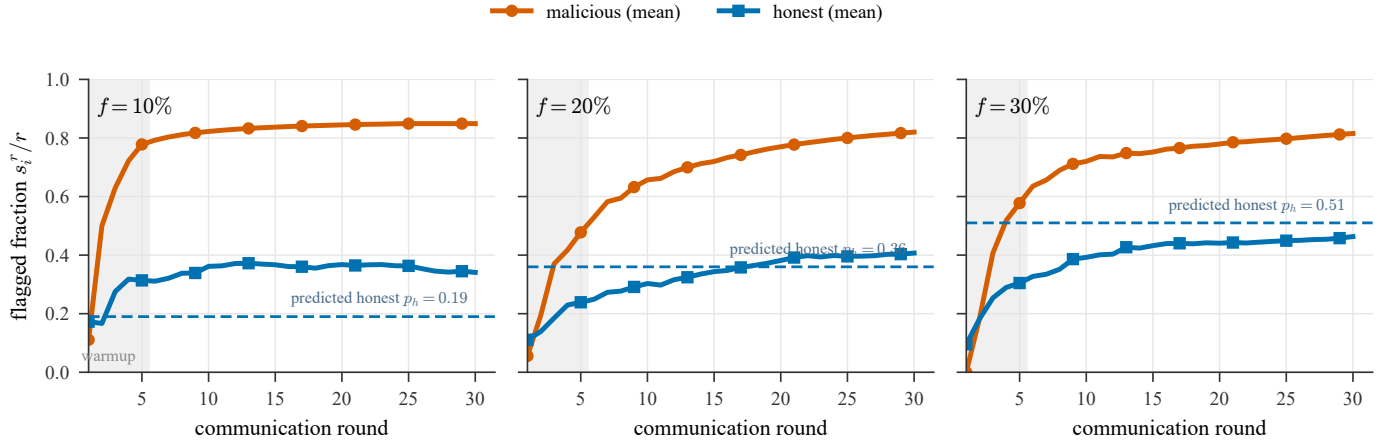
Fig. 9. Temporal suspicion separation (CB-SAFE+ on CIFAR-10): population-mean flagged fraction s_i^r / r of malicious versus honest clients over rounds, for each malicious fraction f (mean over 3 seeds). The two populations separate within a few rounds, so attackers are identified from group-level observations alone (Eqs. (4)–(6)). The dashed line is the predicted honest co-clustering rate p_h = 1 - (1 - f)^{c-1} (Eq. (5)); the loss probe adds a few honest flags at low f . Exclusion uses an adaptive gap between the two populations rather than a fixed threshold; the warmup window is shaded.
