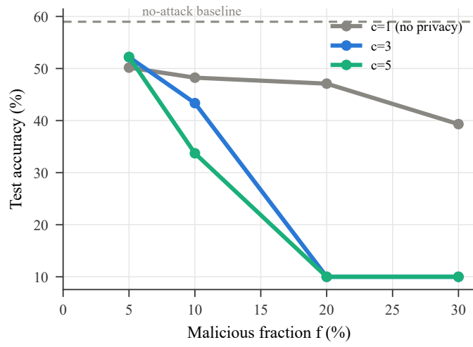
Fig. 10. The privacy–robustness dial, measured: median-rule accuracy under sign-flip for c \in \{1, 3, 5\} . Larger anonymity sets shift the breakdown frontier left, as (1 - f)^c predicts; at f=5\% privacy costs nothing.
