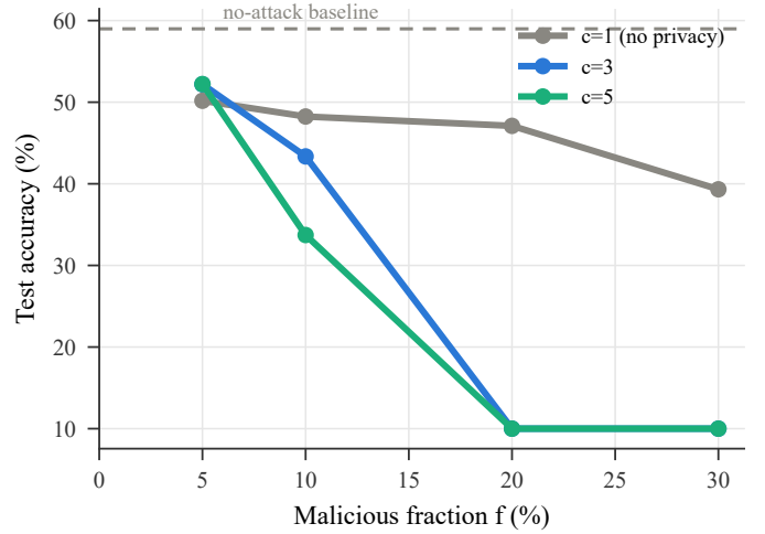
Fig. 7. The privacy–robustness dial, measured: median-rule accuracy under sign-flip for c \in \{1, 3, 5\} . Larger anonymity sets shift the breakdown frontier left, as (1 - f)^c predicts; at f=5\% privacy costs nothing.
