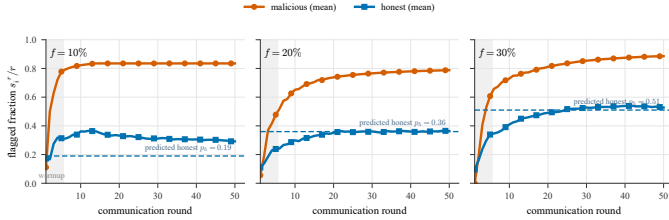
Fig. 7. Temporal suspicion (CB-SAFE+, CIFAR-10): mean flagged fraction s_i^r/r for malicious vs honest clients, per fraction f (3 seeds). Dashed: predicted honest rate p_h = 1 - (1 - f)^{c-1} ; warmup shaded.
