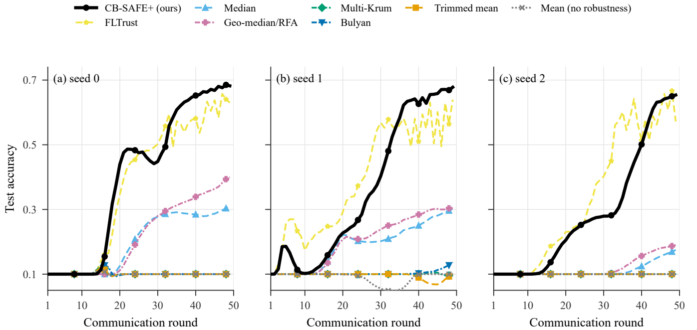
Fig. 3. Test accuracy vs communication round at N=500 (FashionMNIST, sign-flip f=0.2 , 50 rounds), one panel per seed; the eight aggregation rules that admit a configuration at this scale (FedGT excluded, see text).
