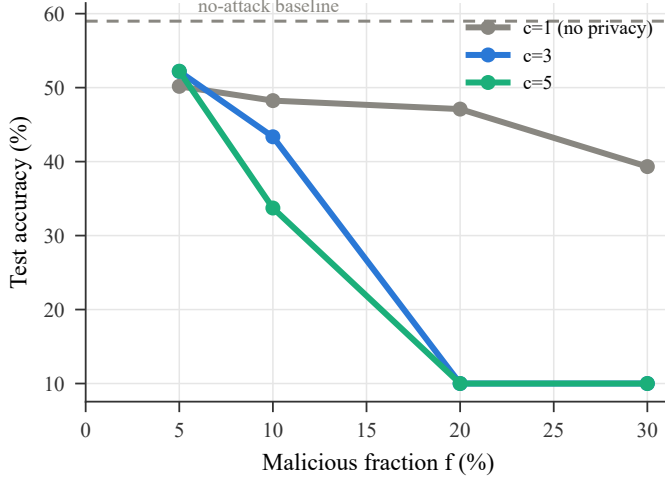
Fig. 7. Privacy-robustness dial: median-rule accuracy under sign-flip for c \in \{1, 3, 5\} (CIFAR-10).
