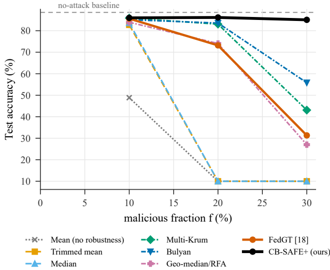
Fig. 7. Sign-flip attack ( \gamma=5 ) on FashionMNIST: test accuracy vs. malicious fraction across eight aggregation rules over k=10 cluster sums ( c=3 , mean of three seeds). Coordinate-wise rules (mean, trimmed mean, median) and the geometric median (RFA) collapse toward chance at the (1-f)^c contamination boundary; vector selection (Multi-Krum, Bulyan) degrades then falls; only CB-SAFE+ holds near the clean baseline across all f , whereas FedGT (its actual BCJR decoder) degrades to \sim 31\% at f=0.3 . All datasets are reported in Table VI.
