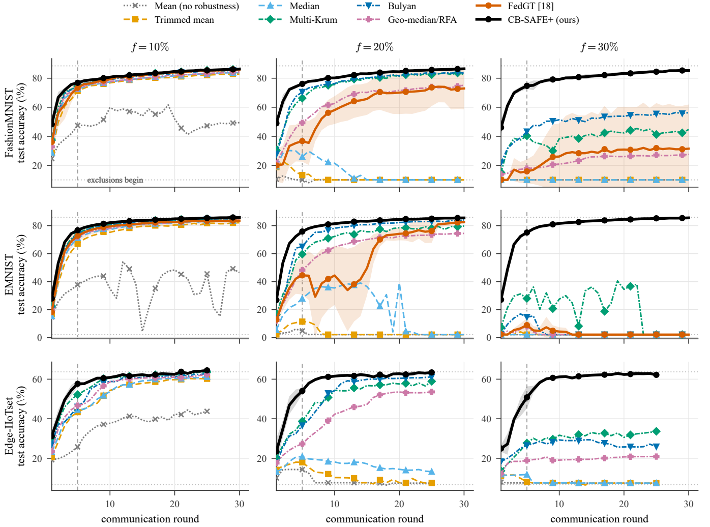
Fig. 9. Training dynamics under the sign-flip attack: test accuracy versus communication round for eight aggregation rules, across three datasets (rows) and malicious fractions f (columns). FedGT is its actual BCJR decoder [18], which has no configuration for Edge-IIoTset and is therefore omitted from that row. Curves are the mean over 3 seeds (single seed for the EMNIST baselines); shaded bands are \pm 1 SD for CB-SAFE+ and FedGT. The dashed vertical marks the warmup W=5 after which exclusions begin; dotted lines mark chance and the no-attack baseline. Coordinate-wise rules and the geometric median decay progressively to chance at f \geq 0.2 ; CB-SAFE+ dips during warmup and then recovers and holds, whereas FedGT degrades and collapses toward chance at f=0.3 by over-excluding honest clients. CIFAR-10 is reported in Table VI.
