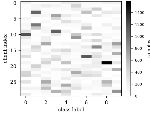
Fig. 3. Non-IID client partition (CIFAR-10, Dirichlet \alpha=0.5 , N=30 ): per-client class-sample counts (darker = more samples). Clients hold 631 to 3298 samples with sharply skewed label distributions, the heterogeneity under which all robustness results are reported.
