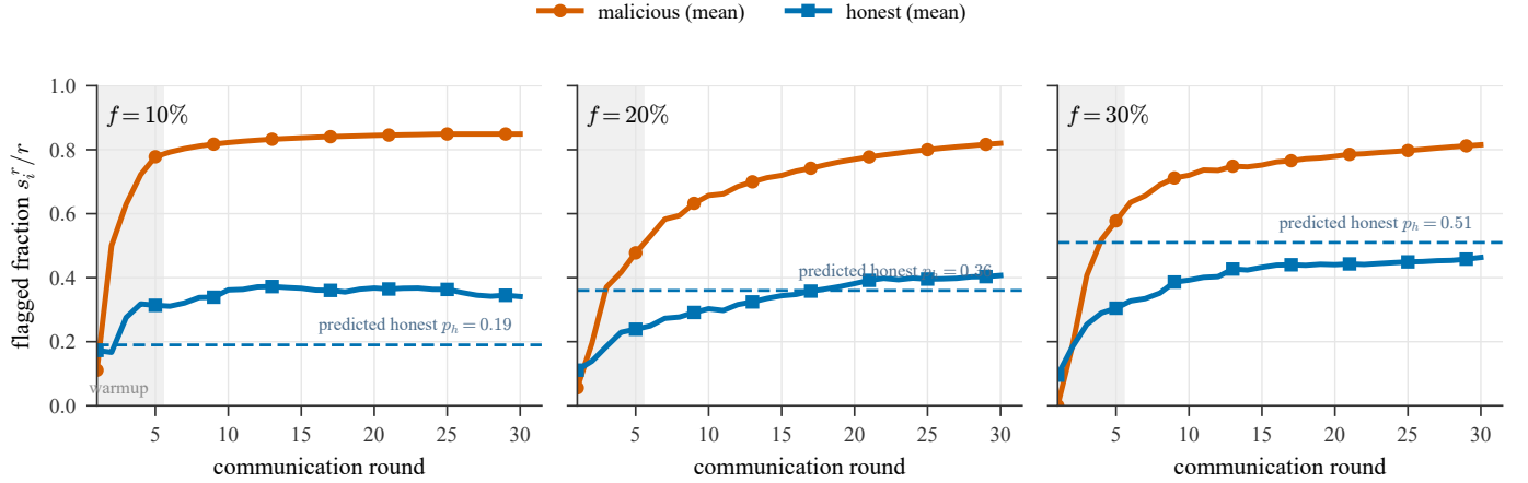
Fig. 7. Temporal suspicion (CB-SAFE+, CIFAR-10): mean flagged fraction s_i^r/r for malicious vs honest clients, per fraction f (3 seeds). Dashed: predicted honest rate p_h = 1 - (1 - f)^{c-1} ; warmup shaded.
