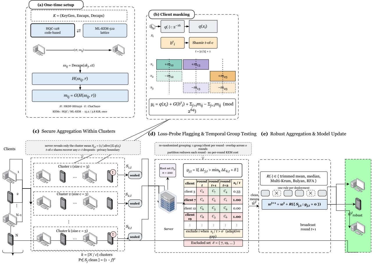
Fig. 1. CB-SAFE, one training round to end: one-time HQC key setup, within-cluster masked aggregation (the server sees only the k cluster sums), and the CB-SAFE+ flag/exclude stage.
