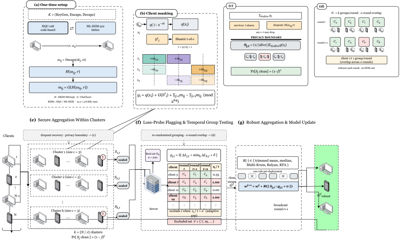
Fig. 1. CB-SAFE end-to-end pipeline: one-time code-based (HQC) key setup, per-round masked cluster aggregation, robust aggregation across cluster sums, and CB-SAFE+ temporal group-testing exclusion.
