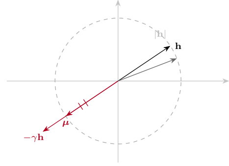
Fig. 2. Laundering geometry (schematic). Averaging c-m honest updates \mathbf{h} with m sign-flips -\gamma\mathbf{h} gives \boldsymbol{\mu} = \frac{c-m(1+\gamma)}{c}\mathbf{h} ; at \gamma^* = 2c/m - 1 it matches |\mathbf{h}| with opposite sign (Proposition 1).
