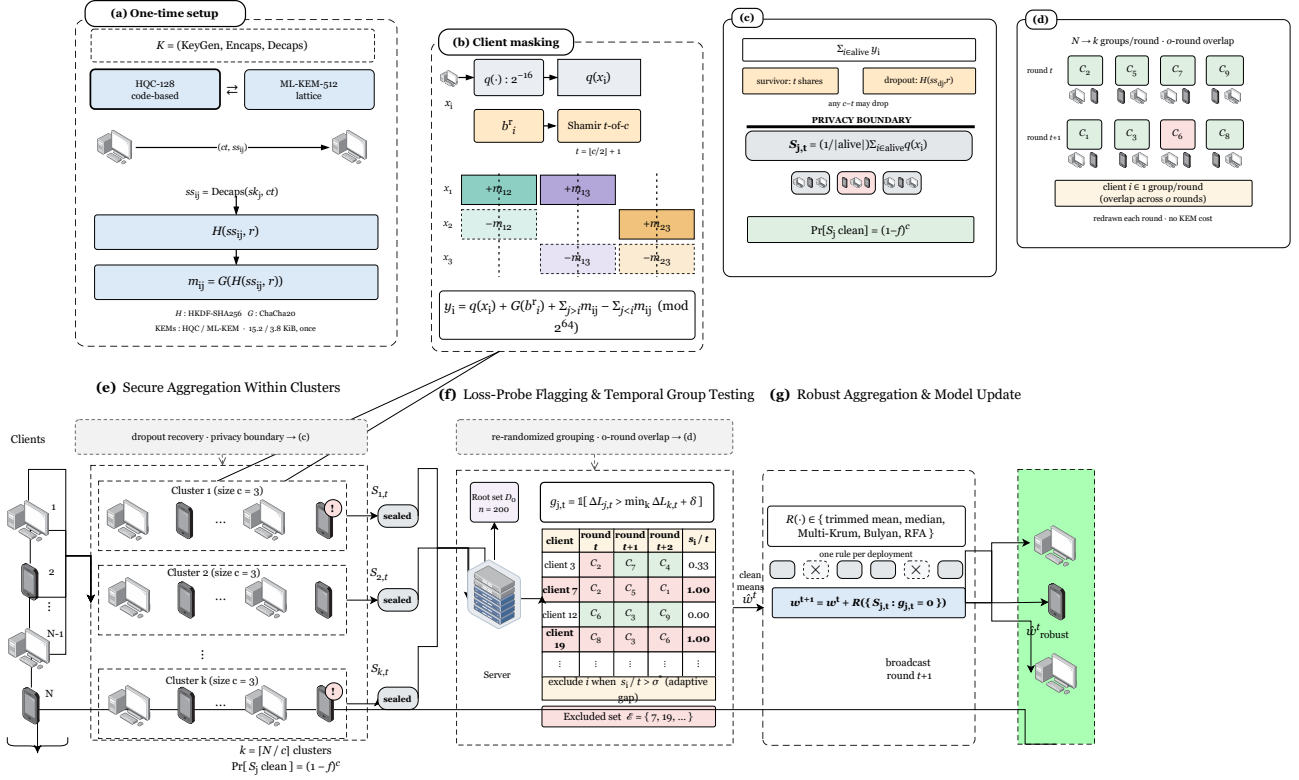
Fig. 1. CB-SAFE, one training round end to end: one-time HQC key setup, within-cluster masked aggregation (the server sees only the k cluster sums), and the CB-SAFE+ flag/exclude stage.
