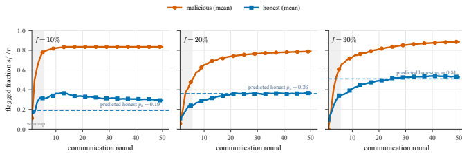
Fig. 7. Temporal suspicion (CB-SAFE+, CIFAR-10): mean flagged fraction s_i^f/r for malicious vs honest clients, per fraction f (3 seeds). Dashed: predicted honest rate p_h = 1 - (1 - f)^{c-1} ; warmup shaded.
