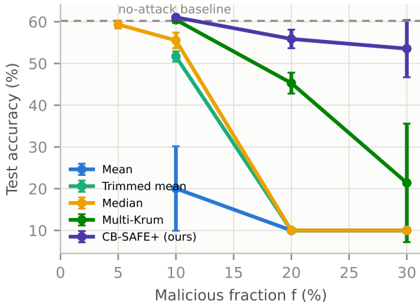
CIFAR-10: sign-flip robustness ( c=3 , 3 seeds)
