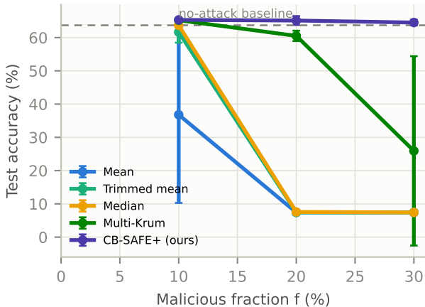
Edge-IIoTset: sign-flip robustness ( c=3 , 3 seeds)
