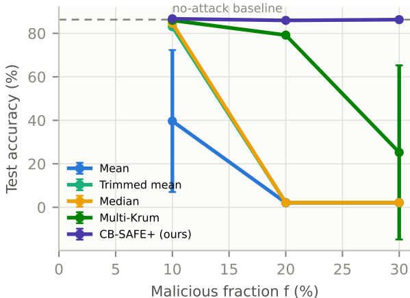
EMNIST: sign-flip robustness ( c=3 , 3 seeds)
