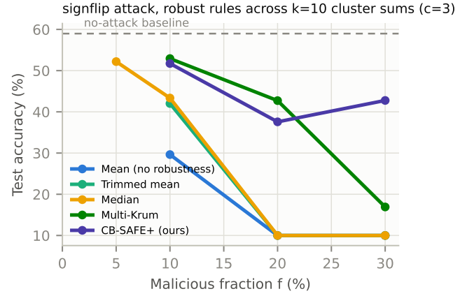
Fig. 6. Sign-flip attack ( \gamma=5 ): accuracy vs. malicious fraction across aggregation rules over k=10 cluster sums ( c=3 ). Coordinate-wise rules collapse at the contamination boundary the (1-f)^c law predicts; vector selection degrades gracefully; CB-SAFE+ identifies and excludes the attackers.
