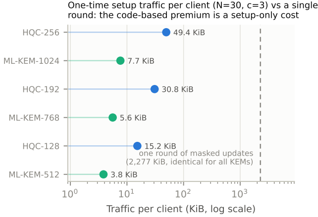
Fig. 4. One-time setup traffic per client versus a single round of masked updates (log scale). Even HQC-256’s setup is \sim 2\% of one round’s traffic; per-round traffic is identical for all KEMs.
