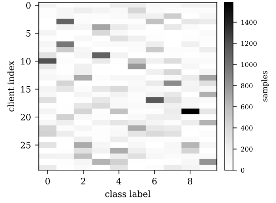
Fig. 3. Non-IID client partition (CIFAR-10, Dirichlet \alpha=0.5 , N=30 ): per-client class-sample counts (darker = more samples). Clients hold 631 to 3298 samples with sharply skewed label distributions, the heterogeneity under which all robustness results are reported.
