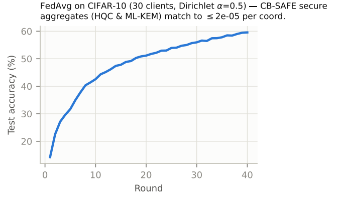
Fig. 5. Test accuracy of FedAvg on non-IID CIFAR-10; CB-SAFE’s secure aggregates (HQC and ML-KEM) are numerically equivalent to plain aggregation, so the accuracy curve is shared by all three configurations.
