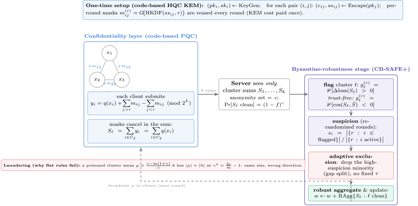
Fig. 1. CB-SAFE, one training round end to end. A one-time code-based (HQC) key setup establishes pairwise secrets reused every round. In the confidentiality layer, clients mask updates so masks cancel within clusters of size c ; the server observes only the k cluster sums (anonymity set c ), never an individual update. The Byzantine-robustness stage (CB-SAFE+) flags clusters by a loss-probe or, in the trust-free variant, a consensus test; accumulates per-client suspicion across re-randomized rounds; adaptively excludes identified attackers; and robustly aggregates the clean cluster sums into the global model, which is broadcast back.
