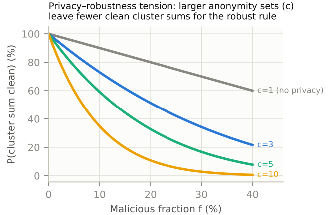
Fig. 10. The privacy–robustness dial, analytically: the anonymity set grows with cluster size c , while the probability that a cluster sum is uncontaminated decays as (1-f)^c .
