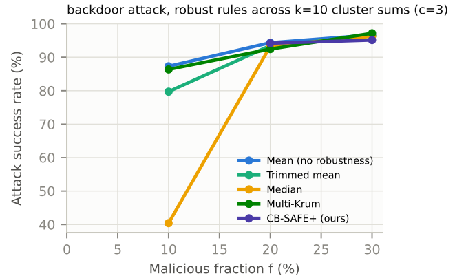
Fig. 7. Backdoor attack success rate vs. malicious fraction. No sum-level rule suppresses the trigger (median at f=0.1 partially excepted): backdoored sums help the main task and evade loss/direction probes, the honest scope limit of robustness under secure aggregation.
