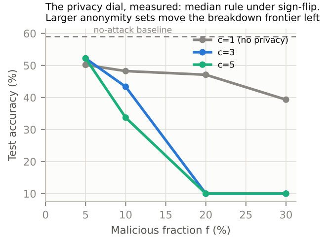
Fig. 9. The privacy–robustness dial, measured: median-rule accuracy under sign-flip for c \in \{1, 3, 5\} . Larger anonymity sets shift the breakdown frontier left, as (1-f)^c predicts; at f=5\% privacy costs nothing.
