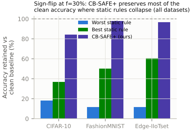
Fig. 8. Sign-flip at f=30\% : fraction of clean-baseline accuracy retained by the worst static rule, the best static rule, and CB-SAFE+, on every dataset. CB-SAFE+ preserves 84–97% where static rules keep 12–60%.
