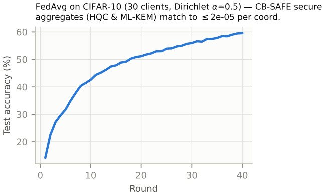
Fig. 3. Test accuracy of FedAvg on non-IID CIFAR-10; CB-SAFE’s secure aggregates (HQC and ML-KEM) are numerically equivalent to plain aggregation, so the accuracy curve is shared by all three configurations.
