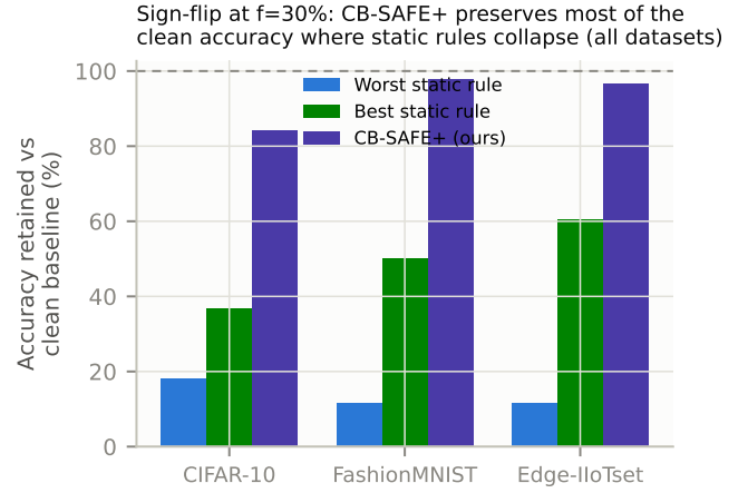
Fig. 6. Sign-flip at f=30\% : fraction of clean-baseline accuracy retained by the worst static rule, the best static rule, and CB-SAFE+, on every dataset. CB-SAFE+ preserves 84–97% where static rules keep 12–60%.
