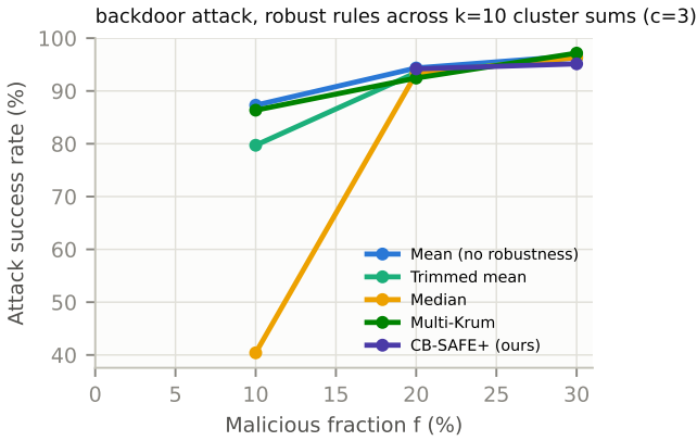
Fig. 5. Backdoor attack success rate vs. malicious fraction. No sum-level rule suppresses the trigger (median at f=0.1 partially excepted): backdoored sums help the main task and evade loss/direction probes, the honest scope limit of robustness under secure aggregation.
