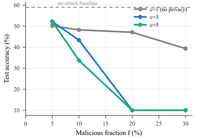
Fig. 9. Privacy-robustness dial: median-rule accuracy under sign-flip for c \in \{1, 3, 5\} (CIFAR-10).
