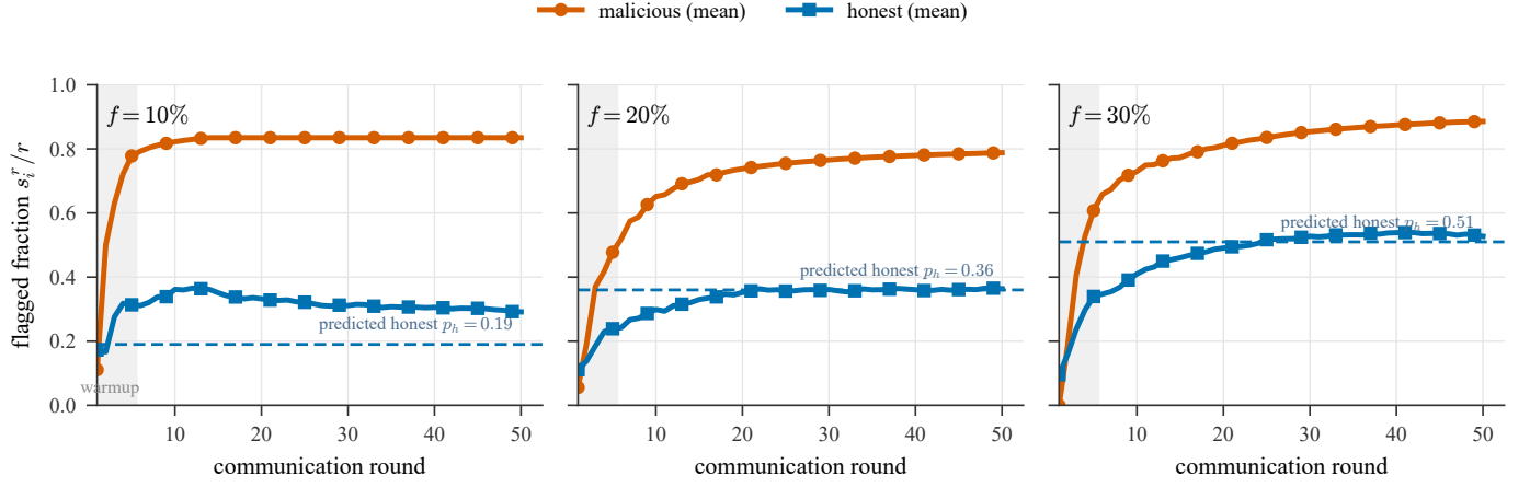
Fig. 8. Temporal suspicion (CB-SAFE+, CIFAR-10): mean flagged fraction s_i^r/r for malicious vs honest clients, per fraction f (3 seeds). Dashed: predicted honest rate p_h = 1 - (1 - f)^{c-1} ; warmup shaded.
