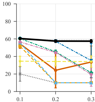
CIFAR-10
