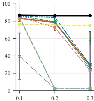
EMNIST
