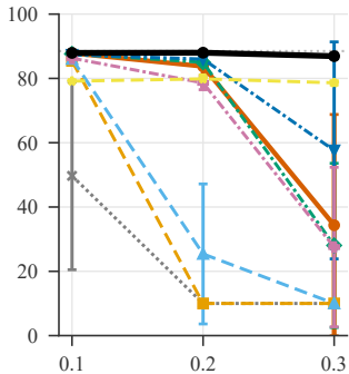
FashionMNIST
